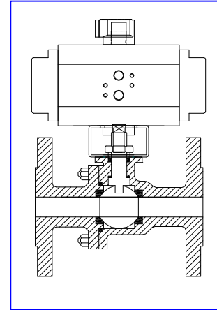
BALL VALVE WITH ROTARY ACTUATOR
