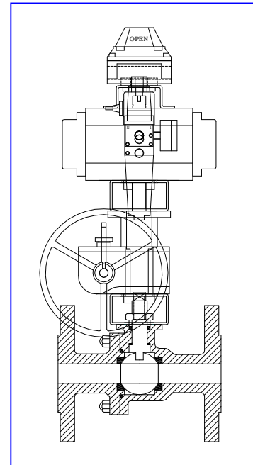
BALL VALVE WITH ROTARY ACTUATOR AND ACCESSORIES
